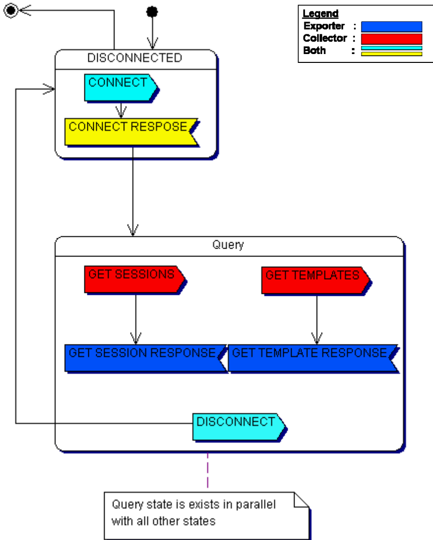
Figure 3: IPDR/SP State Diagram 2
