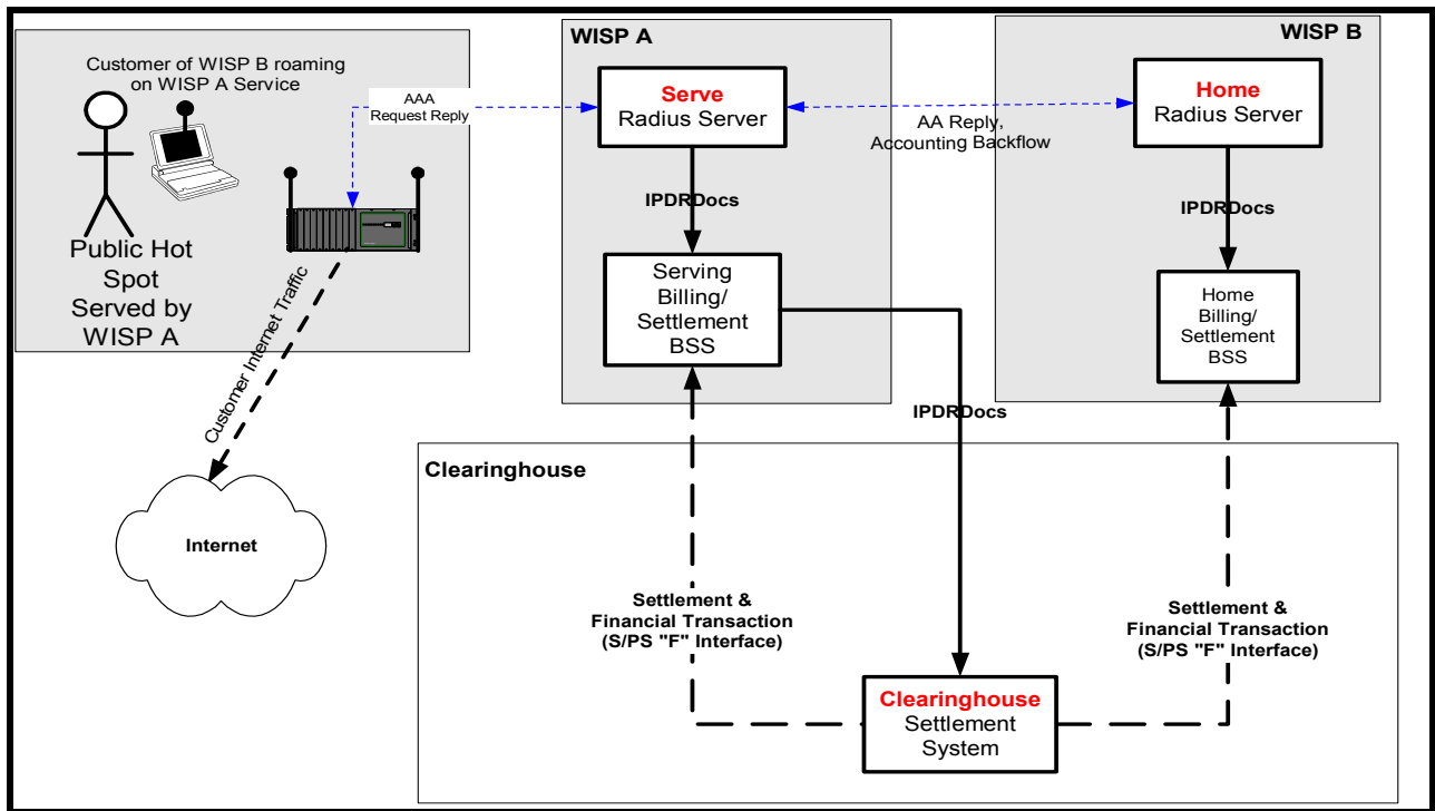
Figure 16 - WiFi Roaming Scenario 2: Clearinghouse and Direct Radius Connection
