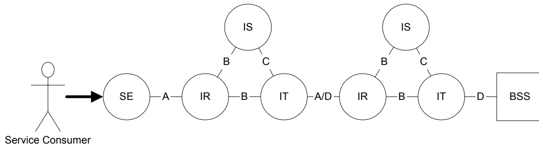
Figure 8: SE Interfaced to BSS via Multiple Mediation Devices
