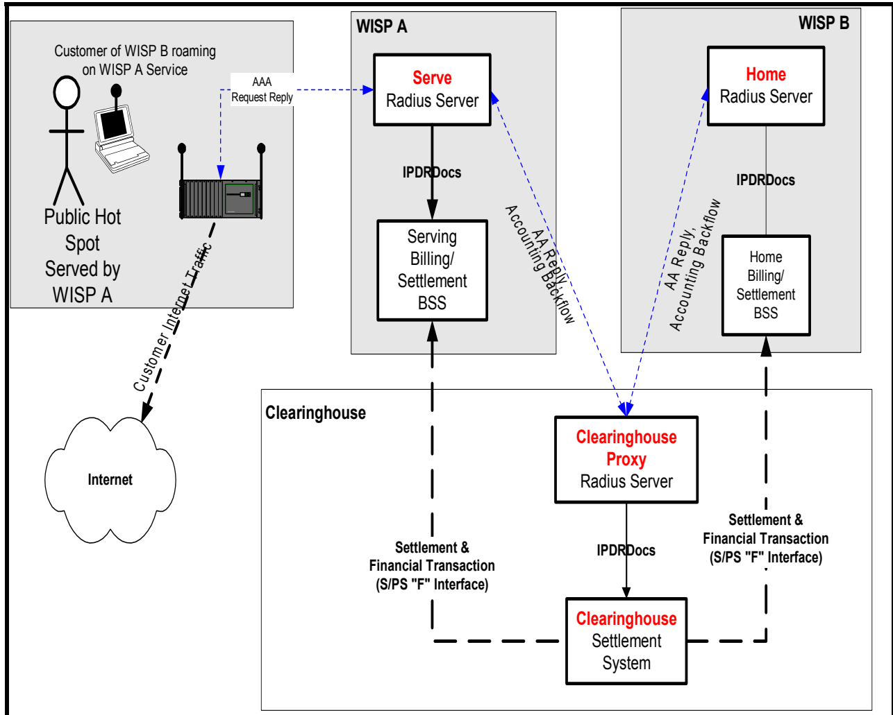
Figure 15 - WiFi Roaming Scenario 1: Clearinghouse with Radius Proxying
