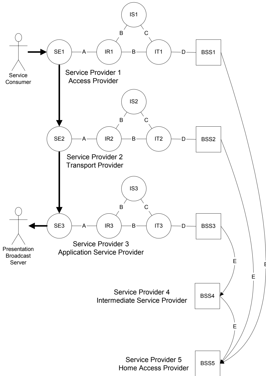
Figure 12: Separate Home, Access, Transport, and Application Service Providers Acting in Concert
